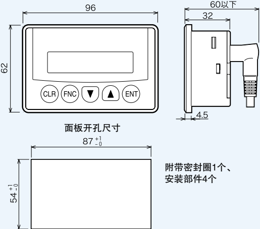
FX-10DM
