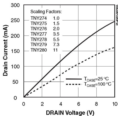
Figure 24. Output Characteristic.
