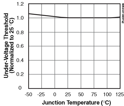
Figure 27. Under-Voltage Threshold vs. Temperature.
