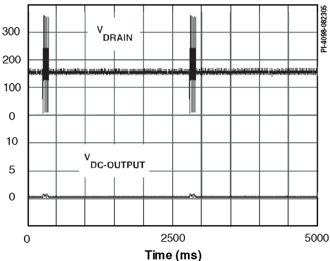
Figure 5. Auto-Restart Operation.
